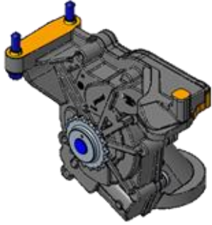
Variable Displacement – Vane Type Oil Pump
